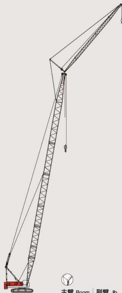
主臂 Boom 副臂 Jib 40m-61m 13m-25m
